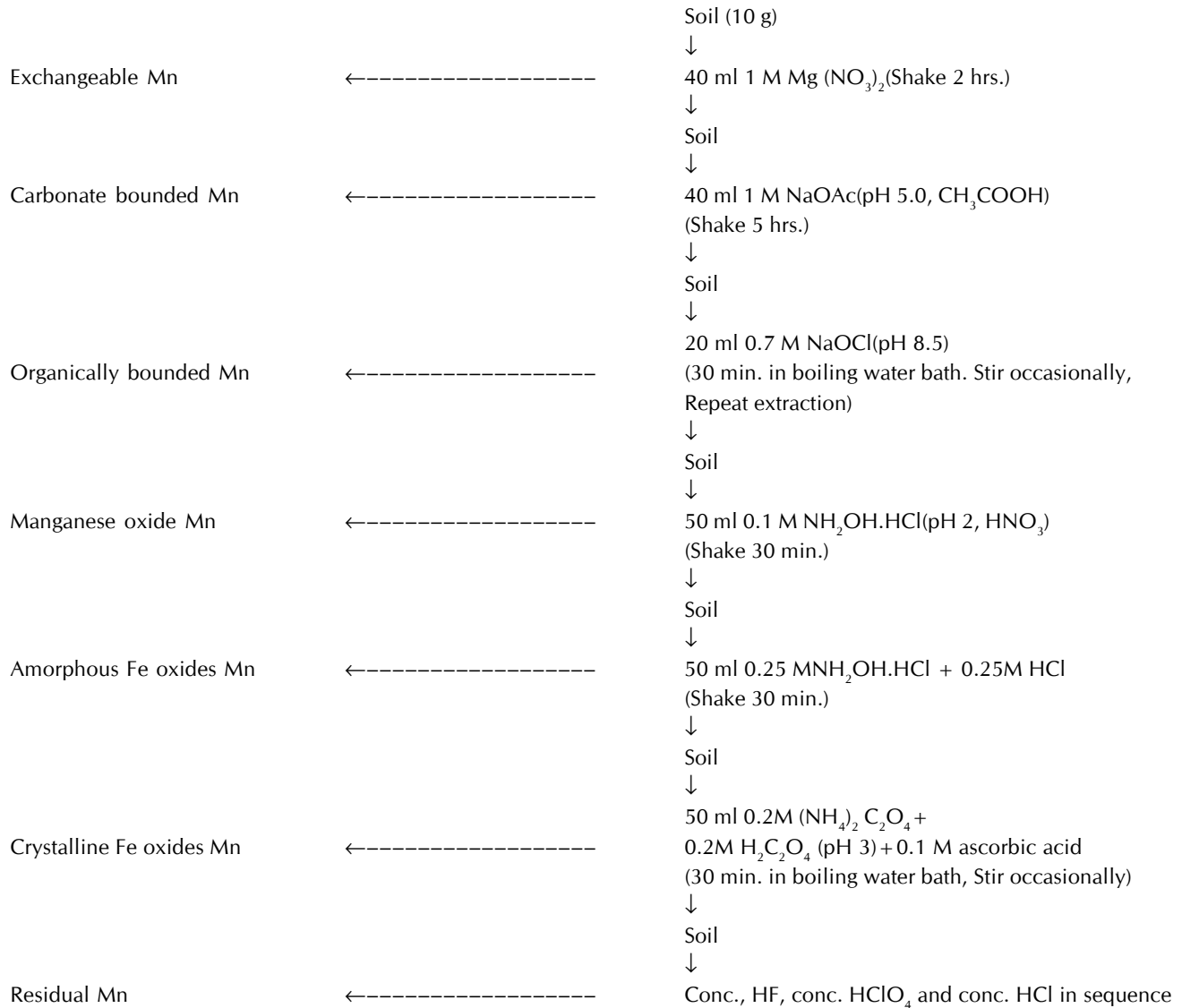
Figure 2: Sequential fractionation scheme for partitioning Mn in soils (Tessier et al. , 1979)
