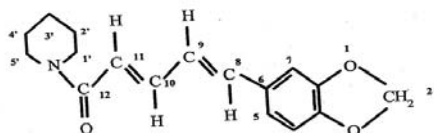
Structure of piperine
